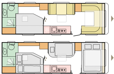
753 UP L 8110 (mm) | W 2460 (mm) | 6
