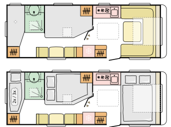
663 UK L 7232 (mm) | W 2460 (mm) | 6+1 opt.
